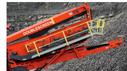
Triple deck Doublescreen with independent screen angle adjustment and screen separation, patent pending
